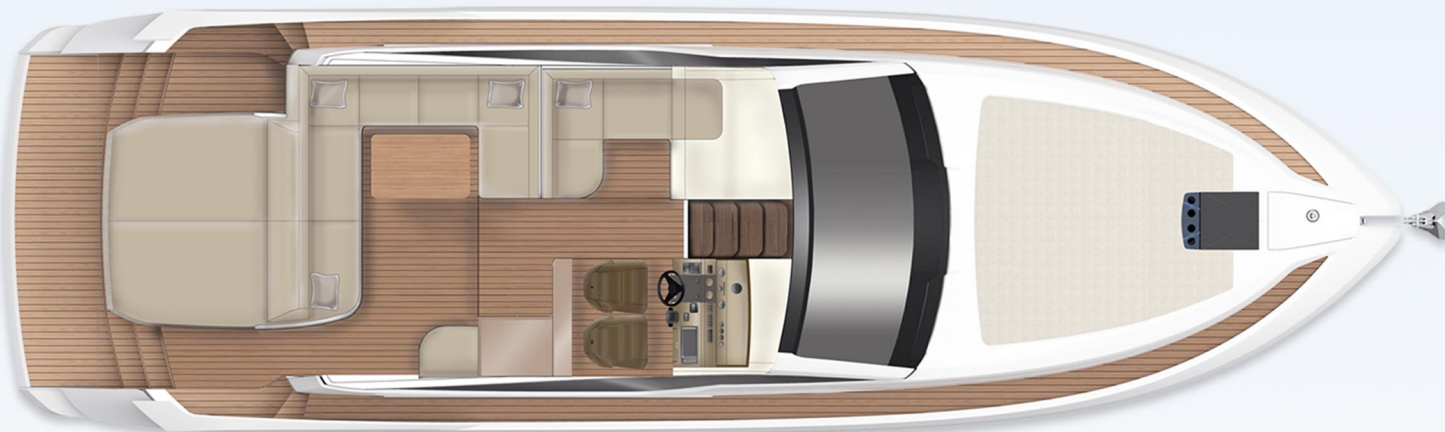
Main Deck
